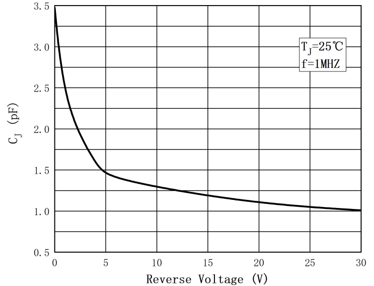
Fig. 2: Capacitance Characteristics
