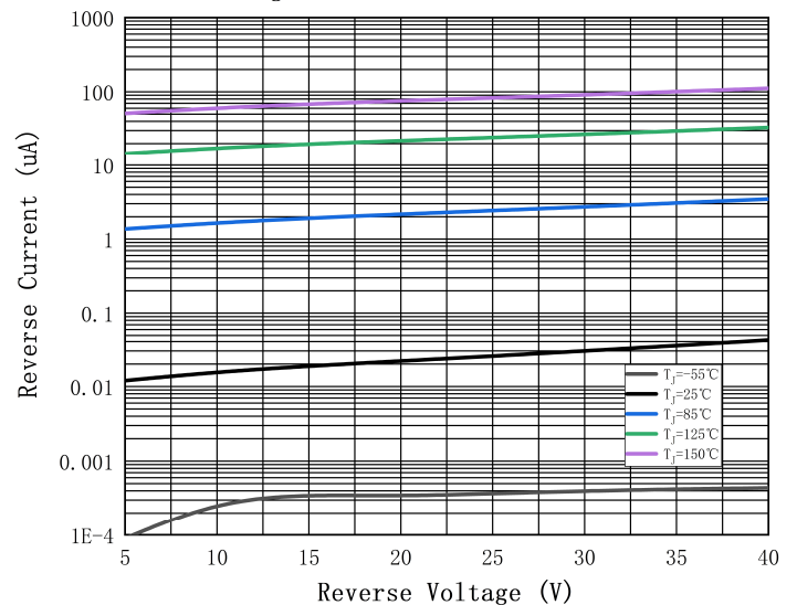
Fig. 4: Reverse Characteristics
