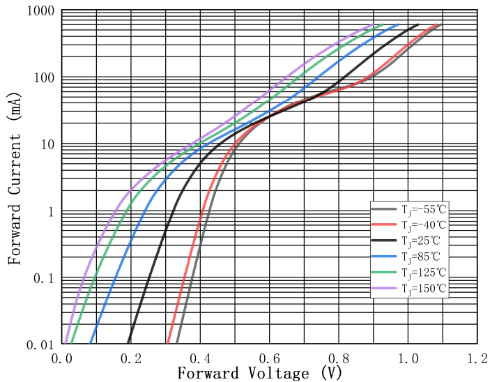
Fig. 3: Forward Characteristics
